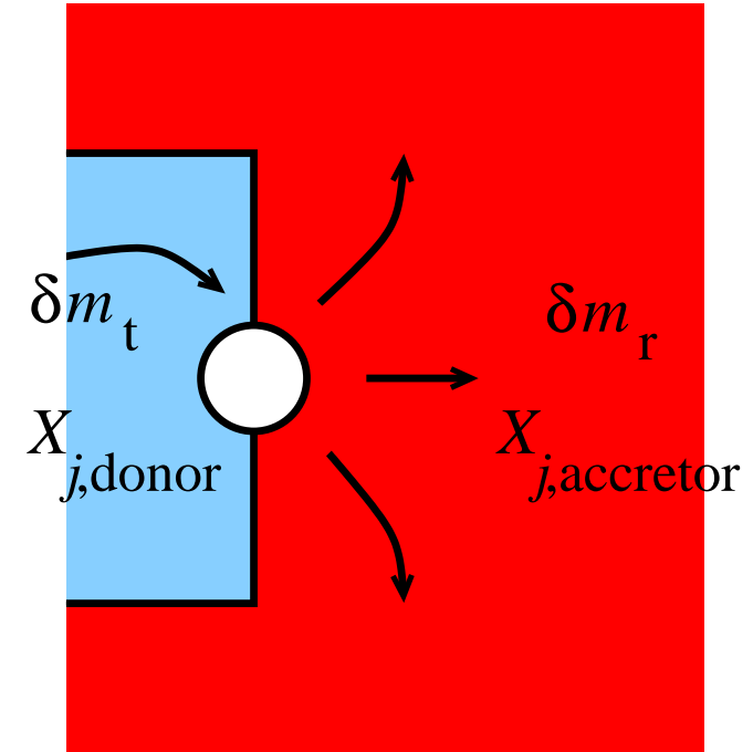
Figure 46: Accretion without interacting winds. Blue represents material from the donor star (not shown) of abundance X_{j,\text{donor}} , red is material from the accreting star of abundance X_{j,\text{accretor}} .
