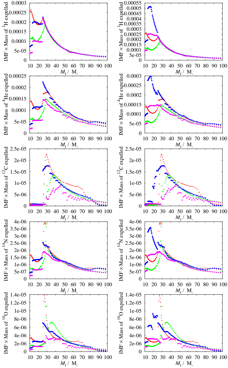
90 Figure 42: Synthetic model massive star wind enrichment modulated by the KTG93 IMF. The left panels show the case for a reduced wind-loss rate ( \times 0.4 for M \leq 25 M_{\odot} ) while the right panels show the standard case. Colours are as in figure 41.
