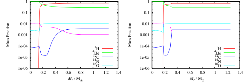
Figure 3: Abundance vs mass co-ordinate M_r inside a 1.25 M_{\odot} , Z = 0.02 star just before and during first dredge-up.
