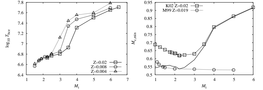
Figure 9: Left panel: Temperature at the base of the convective envelope at the first thermal pulse from the Monash models at various metallicities. Right panel: M_c^{\text{min}} from the Monash models (K02) and the model of Marigo et al. (1999). The solid line shows the core mass at the first thermal pulse in the Monash models.
