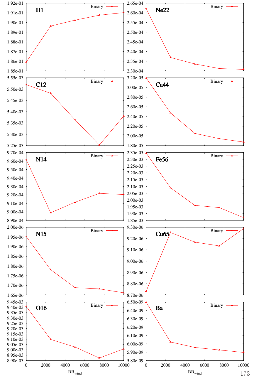
Figure 75: Yield relative to mass input y vs the enhanced binary wind loss factor B .
