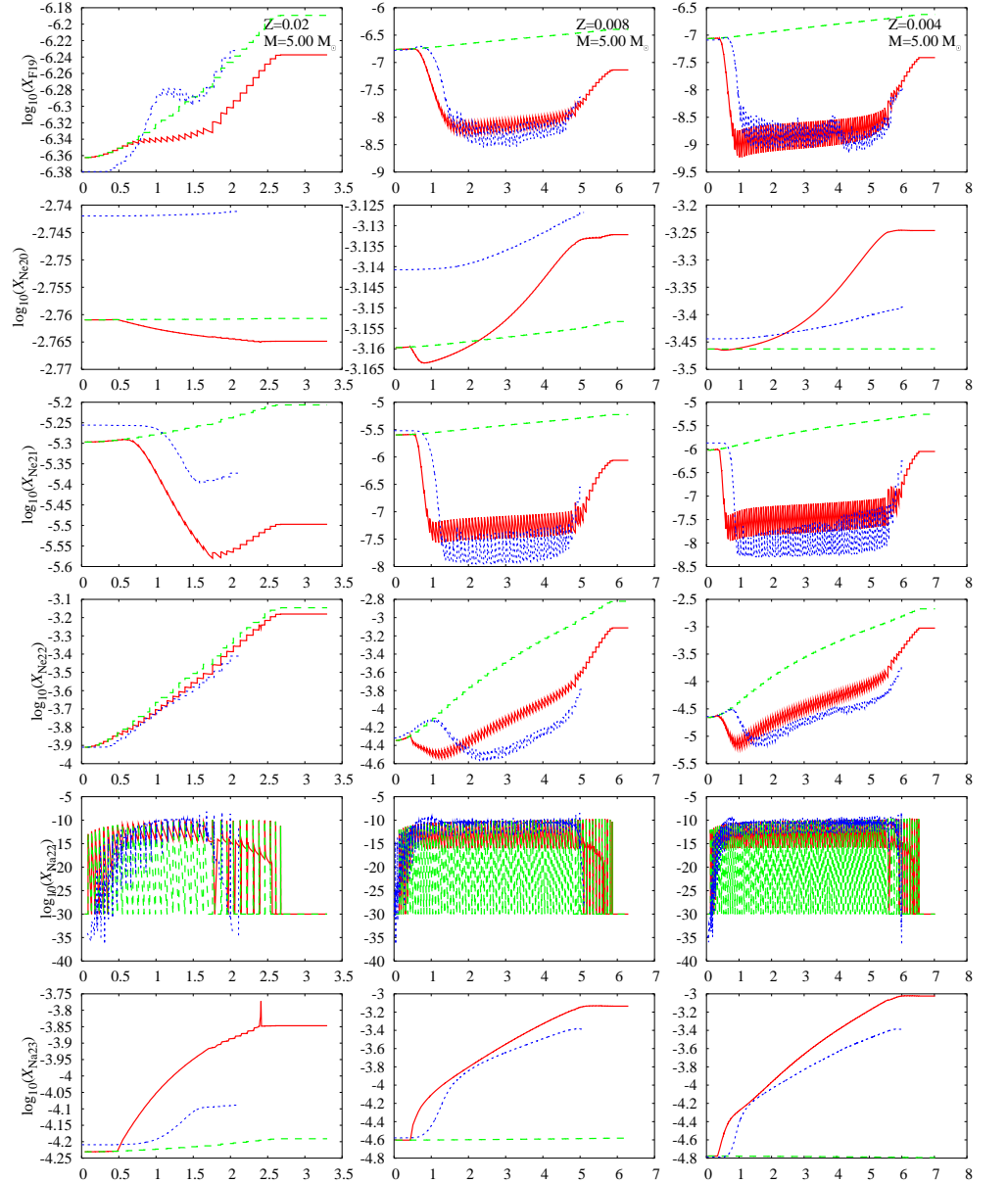
Figure 21: ^{19}\text{F} , ^{20}\text{Ne} , ^{21}\text{Ne} , ^{22}\text{Ne} , ^{22}\text{Na} and ^{23}\text{Na} vs time (in units of 10^5 years) for the 55 synthetic models with NeNa cycling (red), synthetic models without NeNa cycling (green) and the Monash models (blue) M = 5 M_{\odot} . Note that when the red lines are invisible they are hiding under the green lines.
