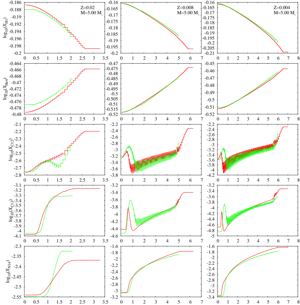
Figure 13: ^1\text{H} , ^4\text{He} , ^{12}\text{C} , ^{13}\text{C} and ^{14}\text{N} vs time (in units of 10^5 years) for the synthetic models (red) and the Monash models (green) with M = 5M_{\odot} .
