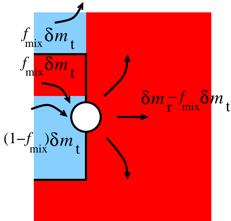
Figure 47: As Fig. 46 with interacting winds. A fraction f_{\text{mix}} of the donor's material (blue) mixes with the wind (red) prior to accretion.
