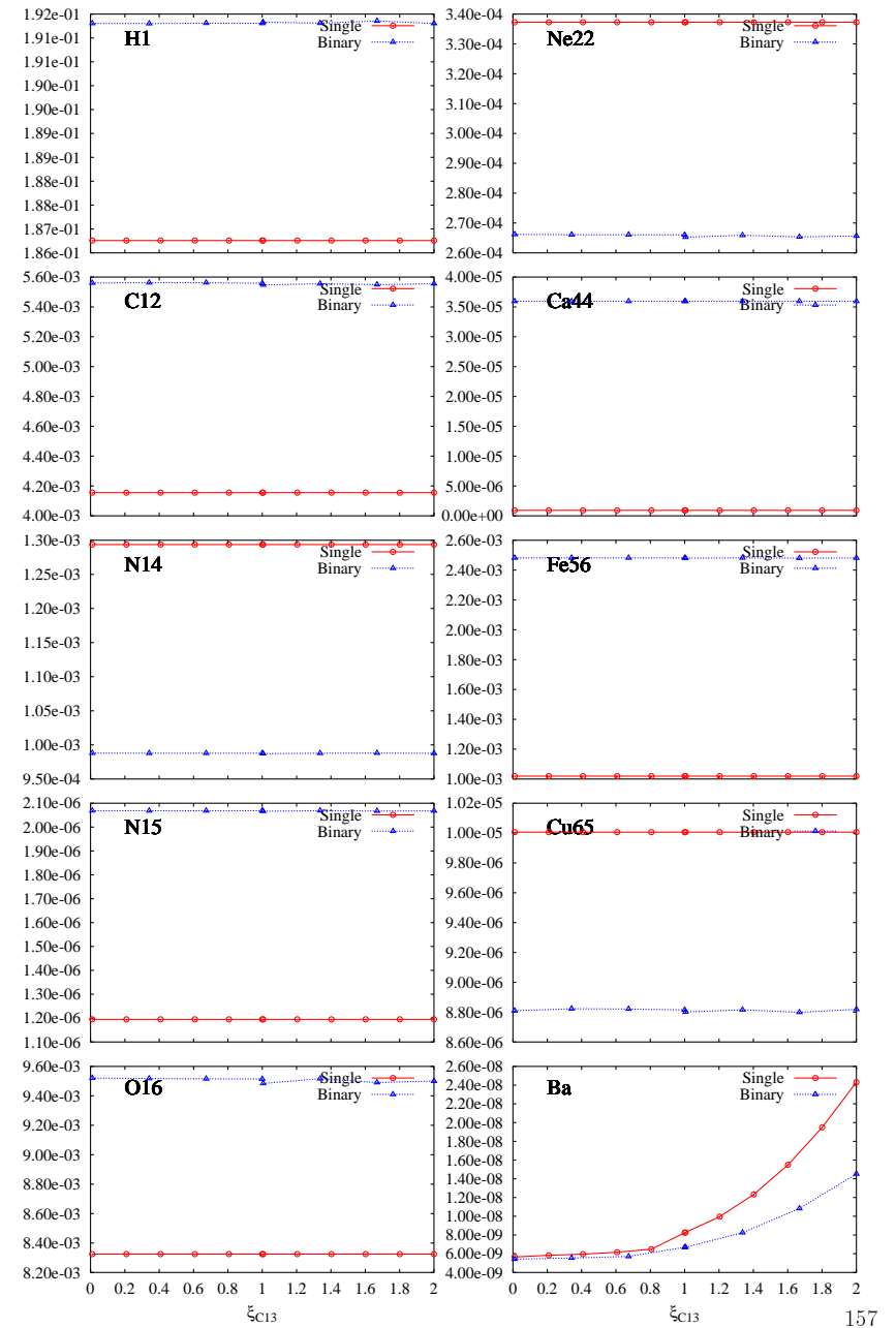
Figure 67: Yield relative to mass input y vs s -process pocket efficiency.
