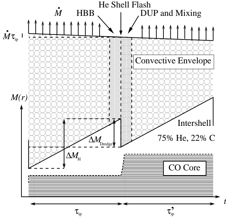
Figure 5: Time evolution of the synthetic AGB model ( \lambda > 0 , not to scale). During the interpulse period \tau_{\text{ip}} the hydrogen-free core M_c (Intershell + CO Core) grows by \Delta M_{\text{H}} and the envelope loses mass \dot{M}\tau_{\text{ip}} . At the end of the interpulse period the envelope is burned using the HBB algorithm and then a He-shell flash occurs causing \Delta M_{\text{dredge}} = \lambda\Delta M_{\text{H}} of material from the Intershell region to mix with the convective envelope. The new interpulse period \tau'_{\text{ip}} is calculated and the evolution continued. The CO core is shown here but is considered to have the same mass as the hydrogen-free core.
