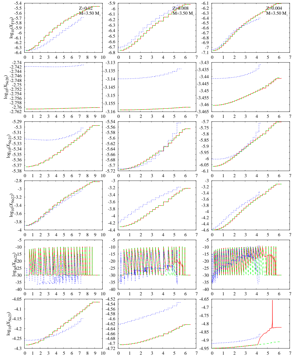
Figure 23: ^{19}\text{F} , ^{20}\text{Ne} , ^{21}\text{Ne} , ^{22}\text{Ne} , ^{22}\text{Na} and ^{23}\text{Na} vs time (in units of 10^5 years) for the 57 synthetic models with NeNa cycling (red), synthetic models without NeNa cycling (green) and the Monash models (blue) M = 3.5 M_{\odot} . Note that when the red lines are invisible they are hiding under the green lines.
