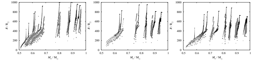
Figure 7: As figure 6 but for radius.
