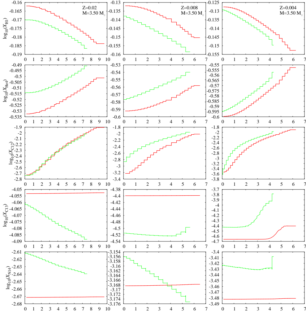
Figure 17: ^1\text{H} , ^4\text{He} , ^{12}\text{C} , ^{13}\text{C} and ^{14}\text{N} vs time (in units of 10^5 years) for the synthetic models (red) and the Monash models (green) with M = 3.5 M_\odot .
