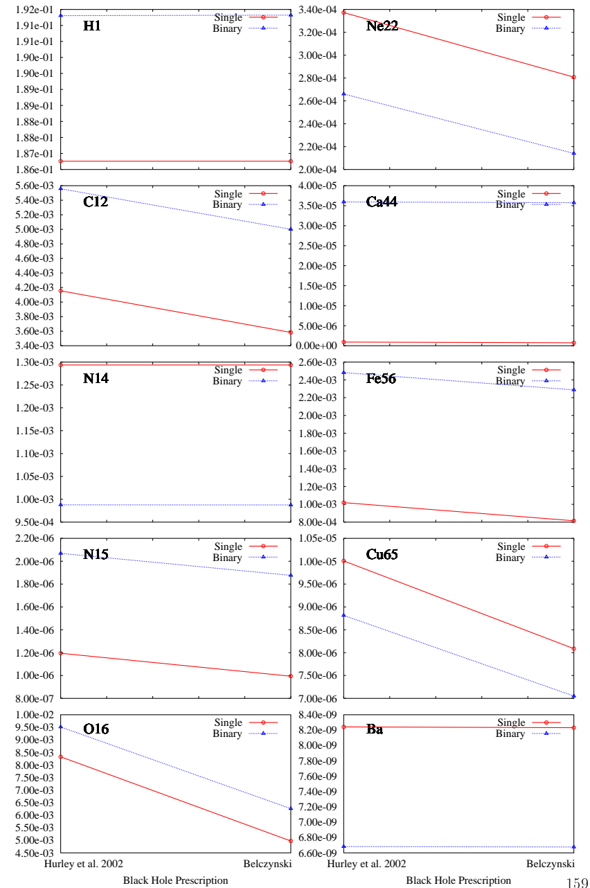
Figure 68: Yield relative to mass input \gamma vs black hole mass prescription.
