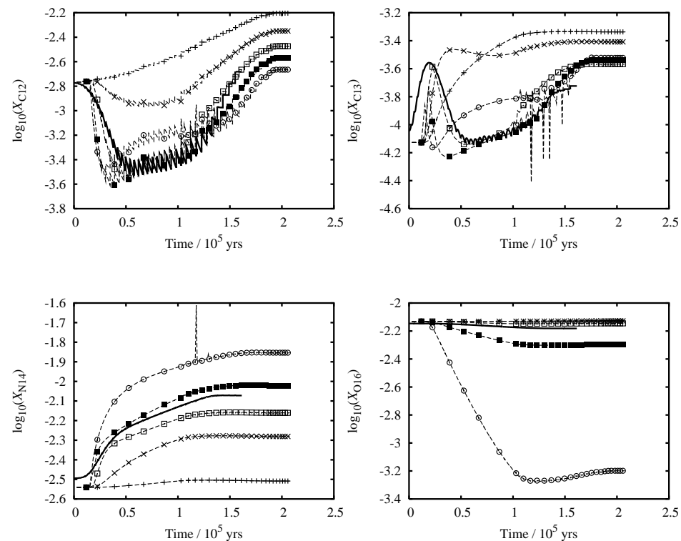
Figure C8: ^{12}\text{C} , ^{13}\text{C} , ^{14}\text{N} and ^{16}\text{O} surface abundances vs time for M_1 = 6 M_\odot , Z = 0.02 with varying temperature factor 0.98 < f_T < 1.02 . The solid line is the corresponding Monash model. The dashed lines represent f_T = 0.98 to 1.02 in 0.01 increments, from top to bottom (+, \times , \square , \blacksquare and \circ respectively). See text for details.
