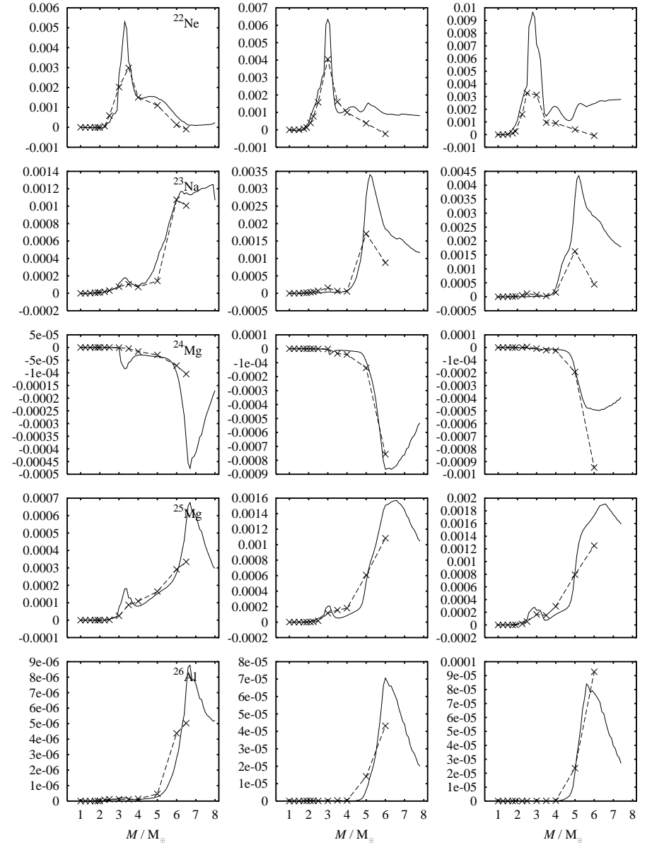
Figure 34: As figure 32 but for ^{22}\text{Ne} to ^{26}\text{Al} .
