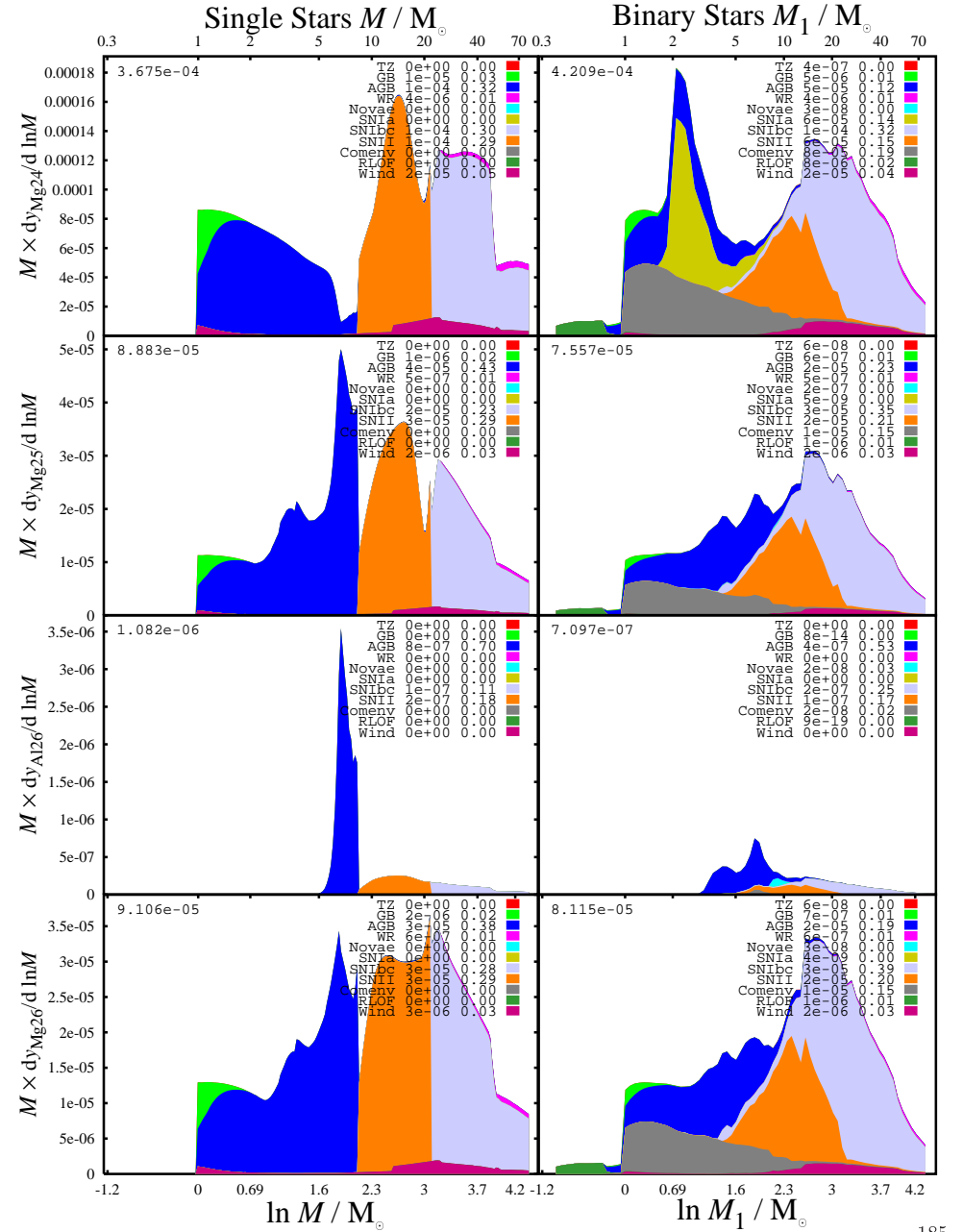
Figure 79: Yield per unit mass input to stars for ^{24}\text{Mg} , ^{25}\text{Mg} , ^{26}\text{Al} and ^{26}\text{Mg} .
