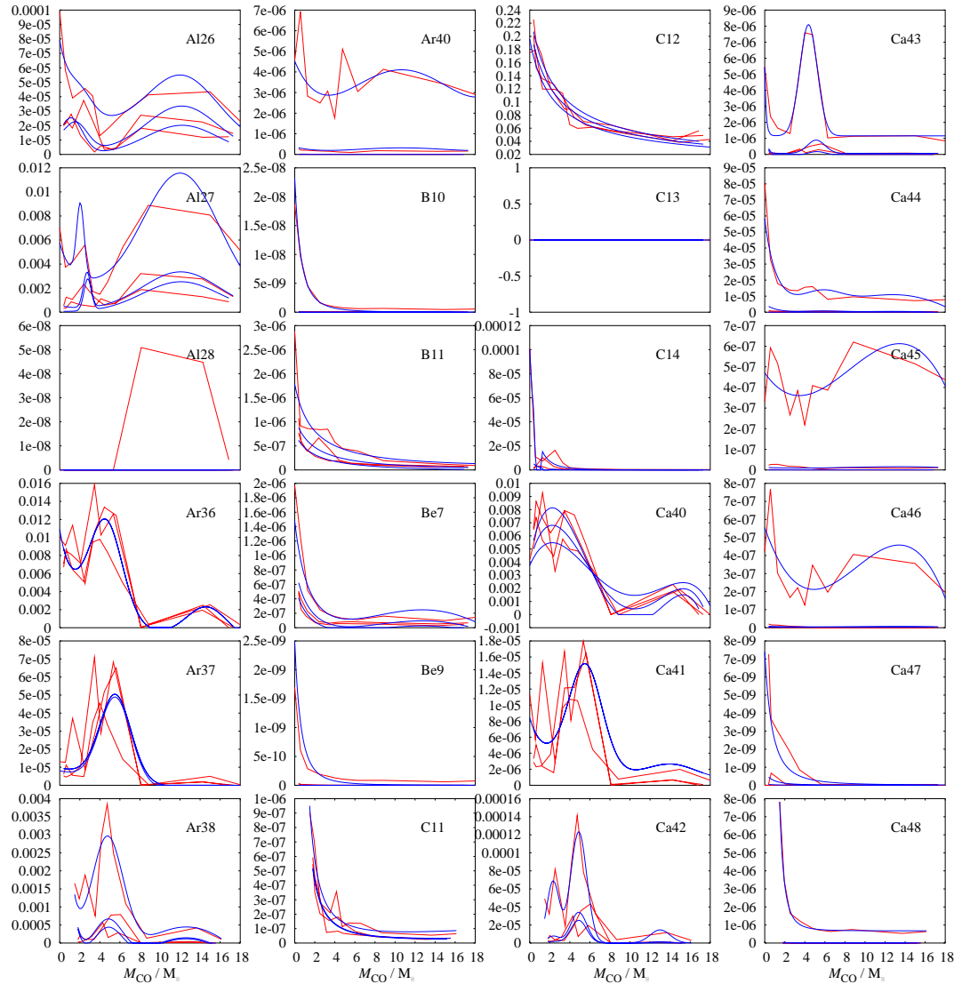
Figure B1: Mass-fraction fits to the WW95 CO core-collapse yields (in alphanumeric order) for ^{26}\text{Al} to ^{48}\text{Ca} . Red lines show the WW95 data, corrected for envelope removal, the blue lines show the fits.
