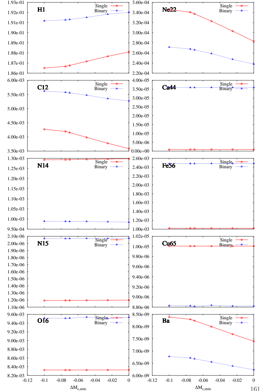
Figure 69: Yield relative to mass input y vs \Delta M_{c,\text{min}} .
