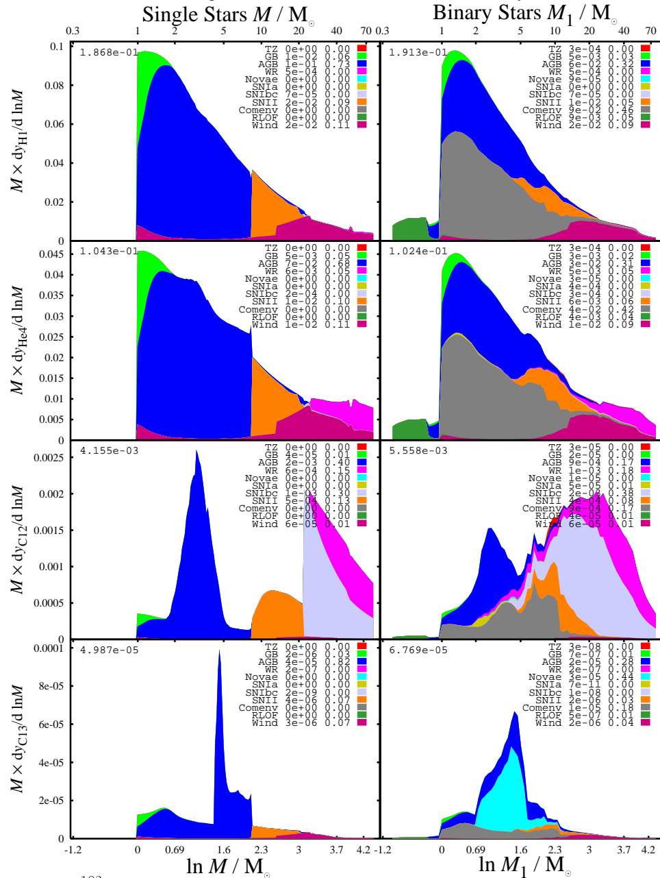
182 Figure 76: Yield per unit mass input to stars y for ^1\text{H} , ^4\text{He} , ^{12}\text{C} and ^{13}\text{C} . See text for details.
