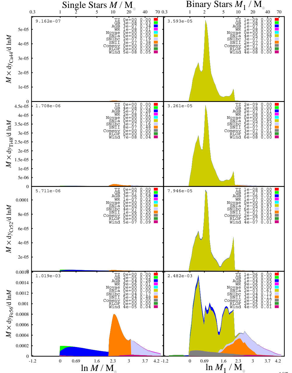
Figure 81: Yield per unit mass input to stars for ^{44}\text{Ca} , ^{48}\text{Ti} , ^{52}\text{Cr} and ^{56}\text{Fe} .
