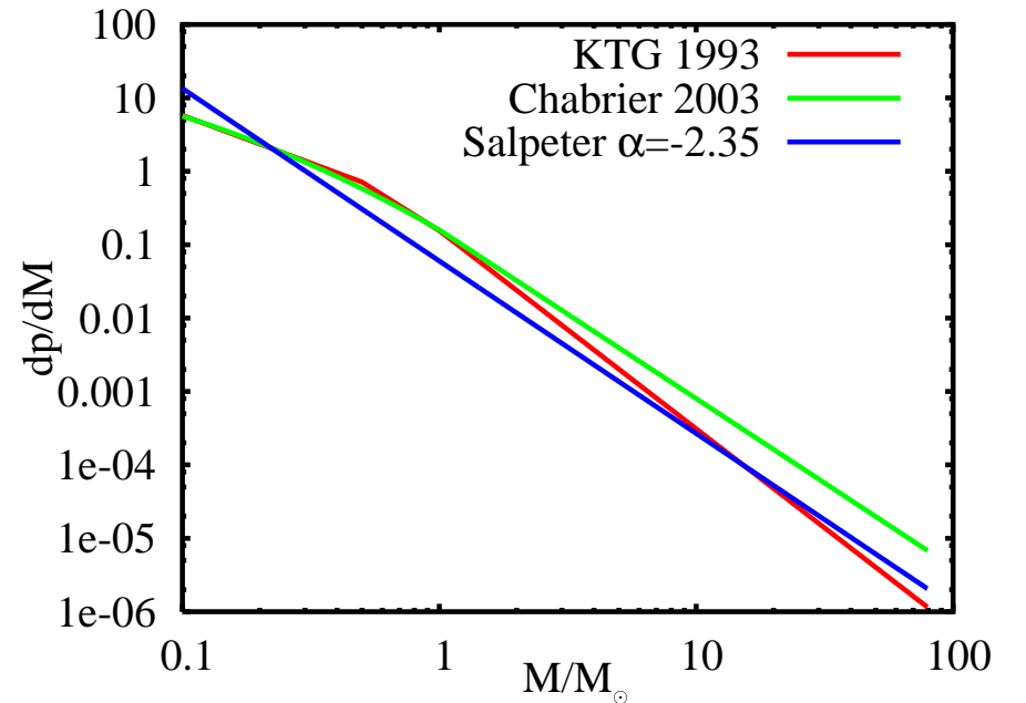
Figure 56: Single star IMFs.
