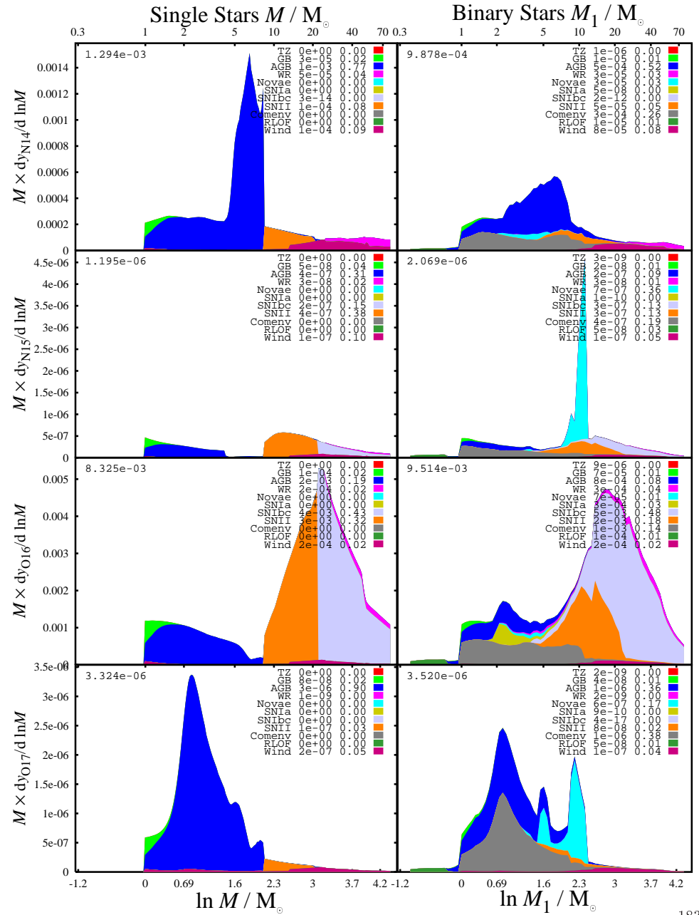
Figure 77: Yield per unit mass input to stars for ^{14}\text{N} , ^{15}\text{N} , ^{16}\text{O} and ^{17}\text{O} .
