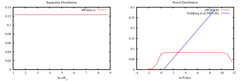
Figure 59: d\Psi/d \ln a and d\Psi/d \ln P generated from a flat- \ln a separation distribution. The blue line is the fit from Goldberg et al. (2003) for the orbital period of spectroscopic binaries.
