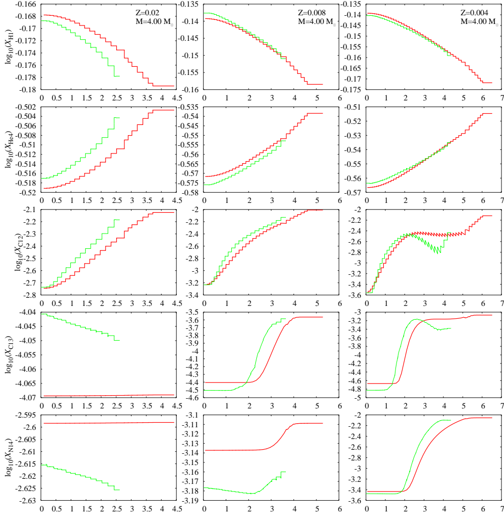
Figure 15: ^1\text{H} , ^4\text{He} , ^{12}\text{C} , ^{13}\text{C} and ^{14}\text{N} vs time (in units of 10^5 years) for the synthetic models (red) and the Monash models (green) with M = 4M_{\odot} .
