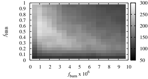
Figure C1: Monte Carlo score (light is best, dark is worst) for varying f_{\text{HBB}} and f_{\text{burn}} when M_i = 6 M_{\odot} , Z = 0.02 . The relation f_{\text{HBB}} \approx (10^6 f_{\text{burn}})^{-1} can be seen to be approximately true.
