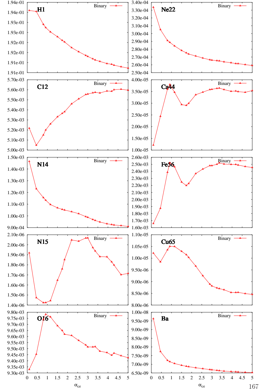
Figure 72: Yield relative to mass input y vs \alpha_{CE} .
