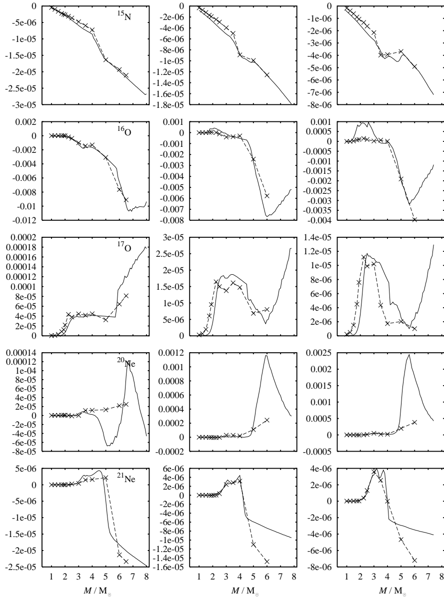
Figure 33: As figure 32 but for ^{15}\text{N} to ^{21}\text{Ne} .
