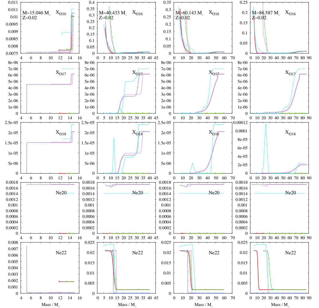
Figure 39: As figure 38 for X_{\text{O16}} , X_{\text{O17}} , X_{\text{O18}} , X_{\text{Ne20}} and X_{\text{Ne22}} . The Dray models do not separate ^{20}\text{Ne} and ^{22}\text{Ne} so all their neon is assumed to be ^{22}\text{Ne} .
