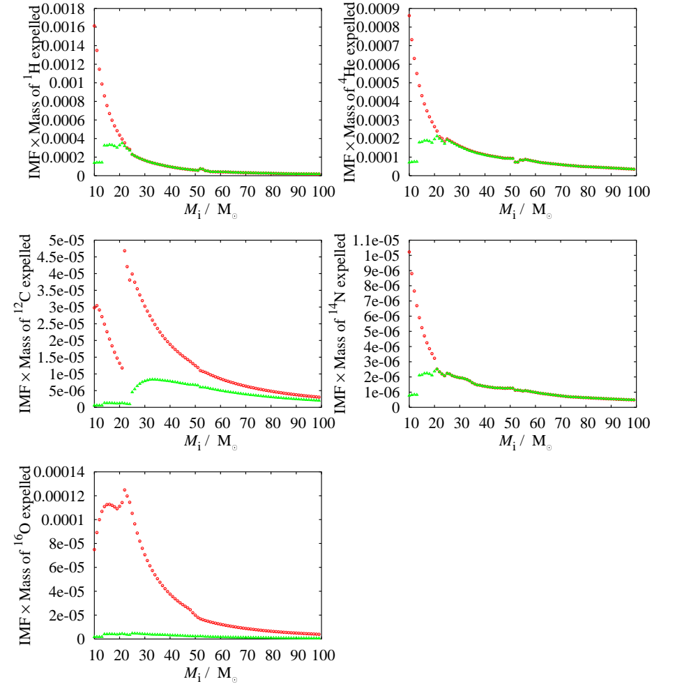
Figure 44: Wind and wind+supernova yields vs initial mass for the Z = 0.02 synthetic model (standard SSE black hole and mass loss prescription, KTG93 IMF weight included). Red is for wind and supernovae, green is wind alone.
