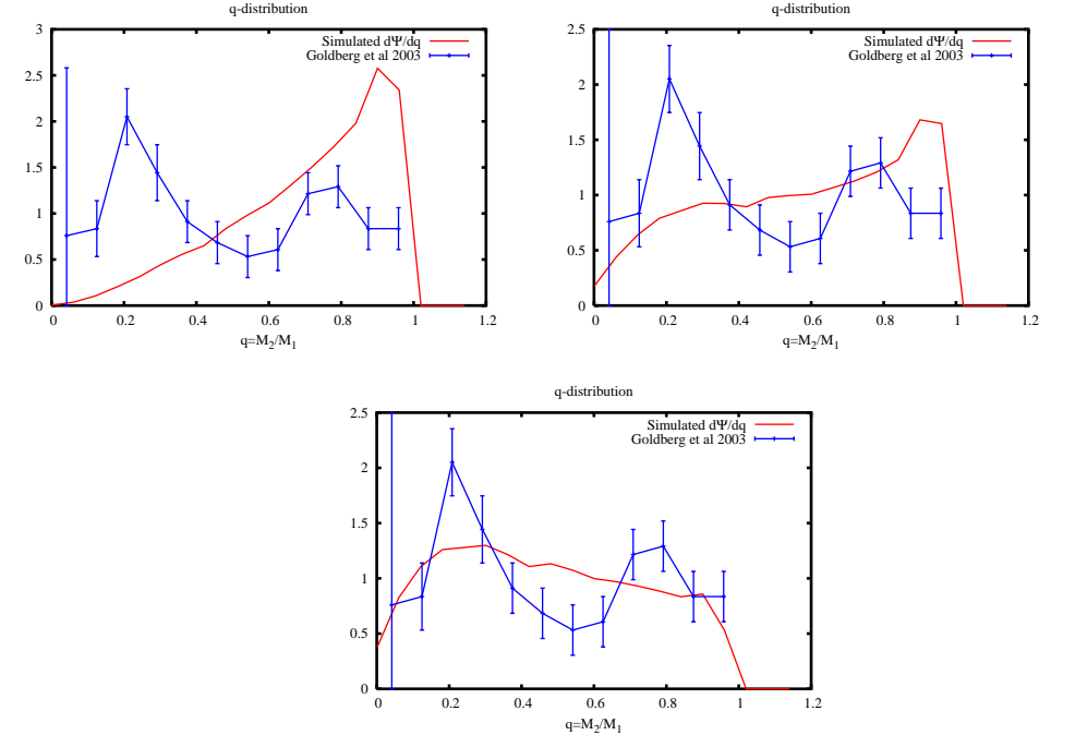
Figure 58: d\Psi/dq vs q (red lines) for \phi(q) \propto q^{0.5} (upper left), \phi(q) \propto q^{-1.5} (upper right) and \psi(M_2) = \psi(M_1) with q \leq 1 (lower panel). The minimum primary mass m_0 = 0.1 .
