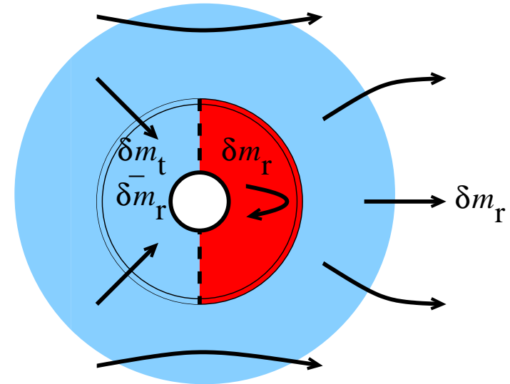
Figure 49: As Fig. 48 with a weak wind and f_{\text{mix}} \leq \delta m_r / \delta m_t . The accreting star accretes a mixture of material from itself and the donor star. Mass \delta m_r is still lost to the ISM but it is all from the donor.
