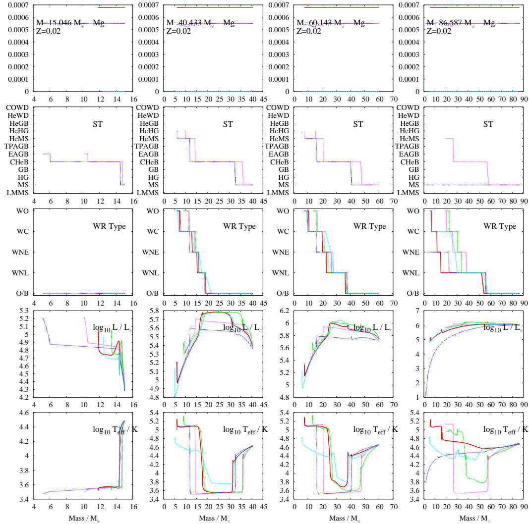
Figure 40: As figure 38 for X_{\text{Mg}24} , the stellar type (defined only for the synthetic models), the WR type, luminosity and effective temperature vs mass.
