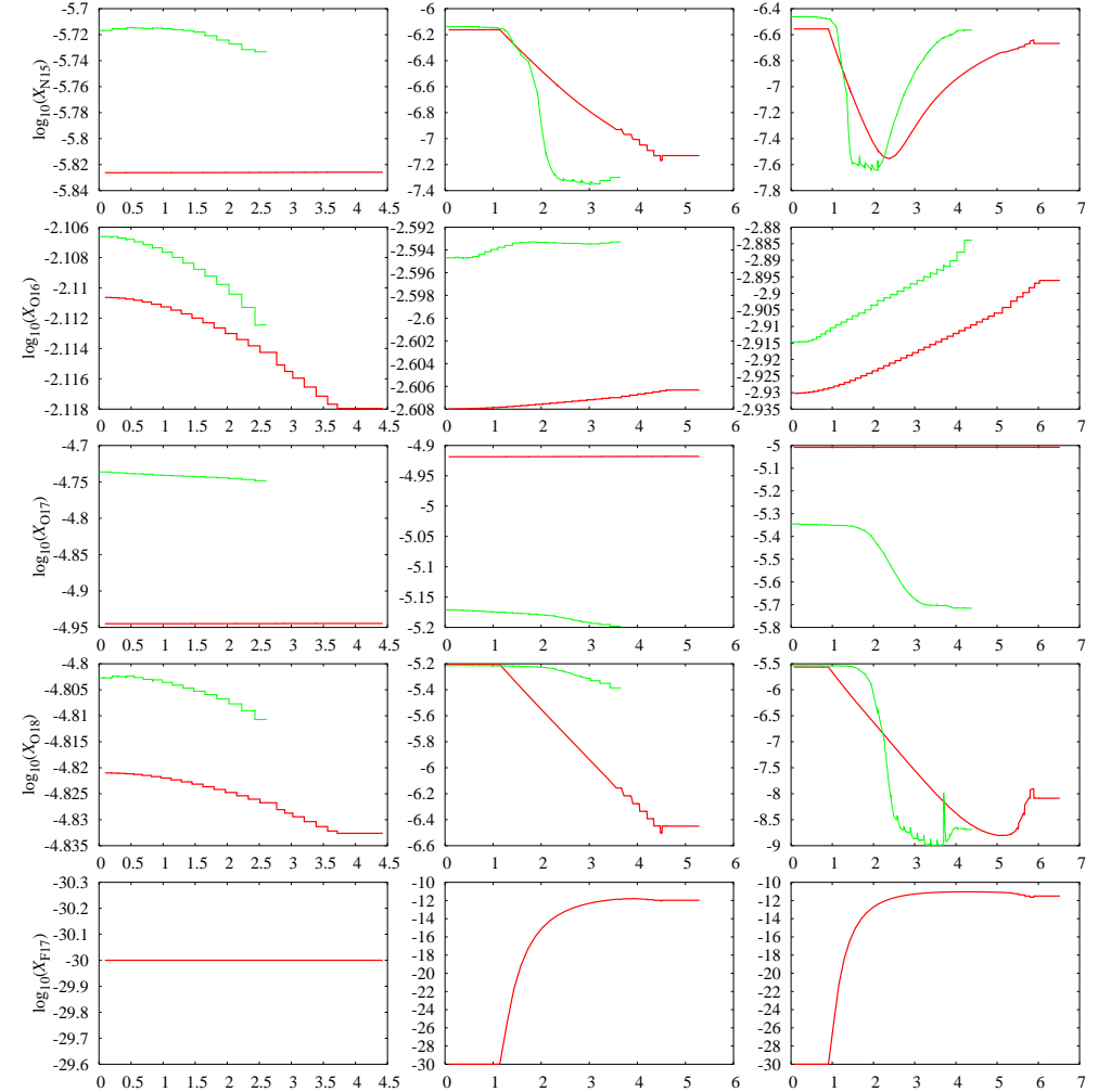
Figure 16: ^{15}\text{N} , ^{16}\text{O} , ^{17}\text{O} , ^{18}\text{O} and ^{17}\text{F} vs time (in units of 10^5 years) for the synthetic models (red) and the Monash models (green) with M = 4M_{\odot} .
