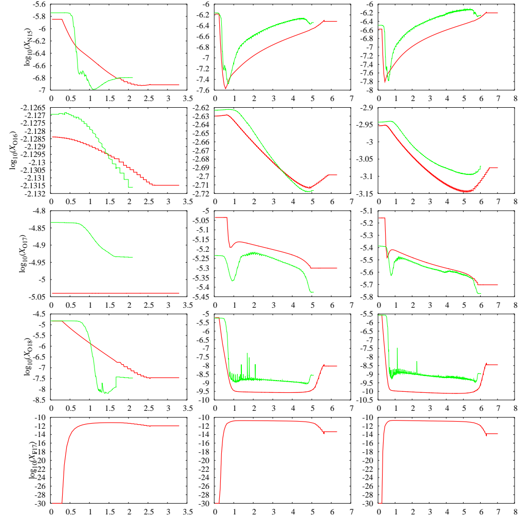
Figure 14: ^{15}\text{N} , ^{16}\text{O} , ^{17}\text{O} , ^{18}\text{O} and ^{17}\text{F} vs time (in units of 10^5 years) for the synthetic models (red) and the Monash models (green) with M = 5M_{\odot} .
