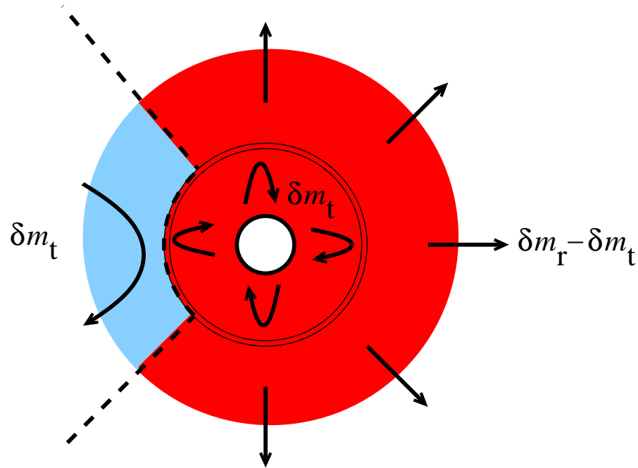
Figure 48: As Fig. 47 with a strong wind and f_{\text{mix}} = 1 . Mass \delta m_t from the donor (blue) is pushed back into space by the accreting star's strong wind. The accreting star still accretes \delta m_t but of its own matter so the surface abundance remains unchanged. The dashed line shows the shock position, not to scale!
