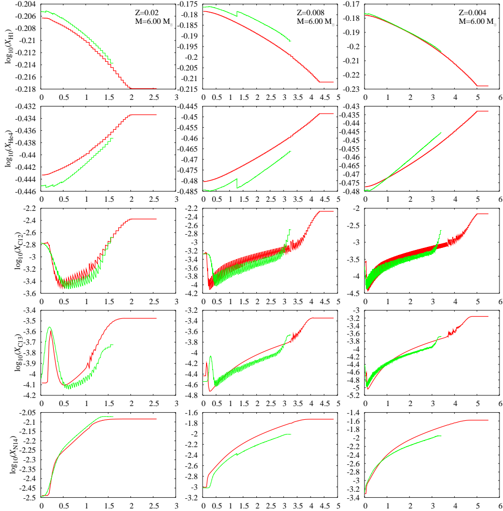
Figure 11: ^1\text{H} , ^4\text{He} , ^{12}\text{C} , ^{13}\text{C} and ^{14}\text{N} vs time (in units of 10^5 years) for the synthetic models (red) and the Monash models (green) with M = 6M_{\odot} .
