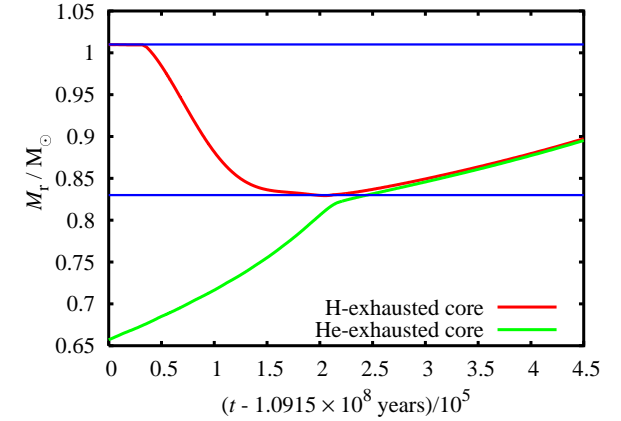
Figure 4: Second dredge-up in a 5 M_{\odot} , Z = 0.02 Eggleton model star. As the He-exhausted core (green line) grows the surface convection zone eats into and shrinks the H-exhausted core (red line). The hydrogen-burned matter between 0.83 and 1.01 M_{\odot} (blue lines) is mixed into the convective envelope, altering surface abundances.
