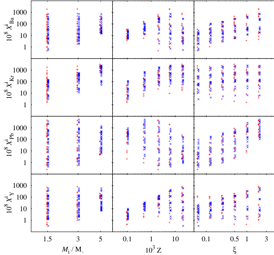
Figure 29: S -process fits (blue) vs FRANEK model data (red) for the key elements Ba, Kr, Pb and Y. The red points have been displaced slightly to the left to be visible. These are projections on M , Z and \xi .
