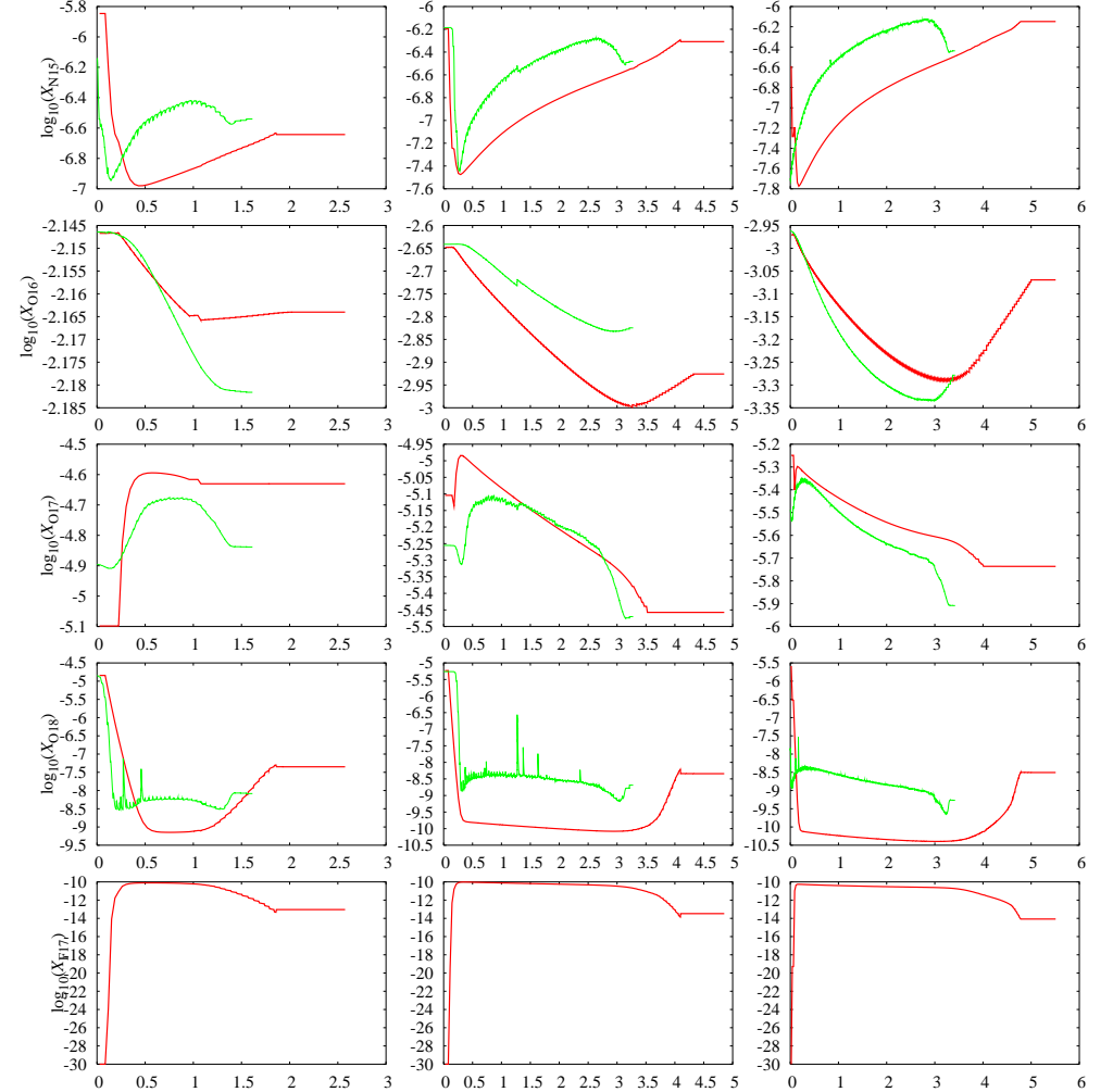
Figure 12: ^{15}\text{N} , ^{16}\text{O} , ^{17}\text{O} , ^{18}\text{O} and ^{17}\text{F} vs time (in units of 10^5 years) for the synthetic models (red) and the Monash models (green) with M = 6M_{\odot} .
