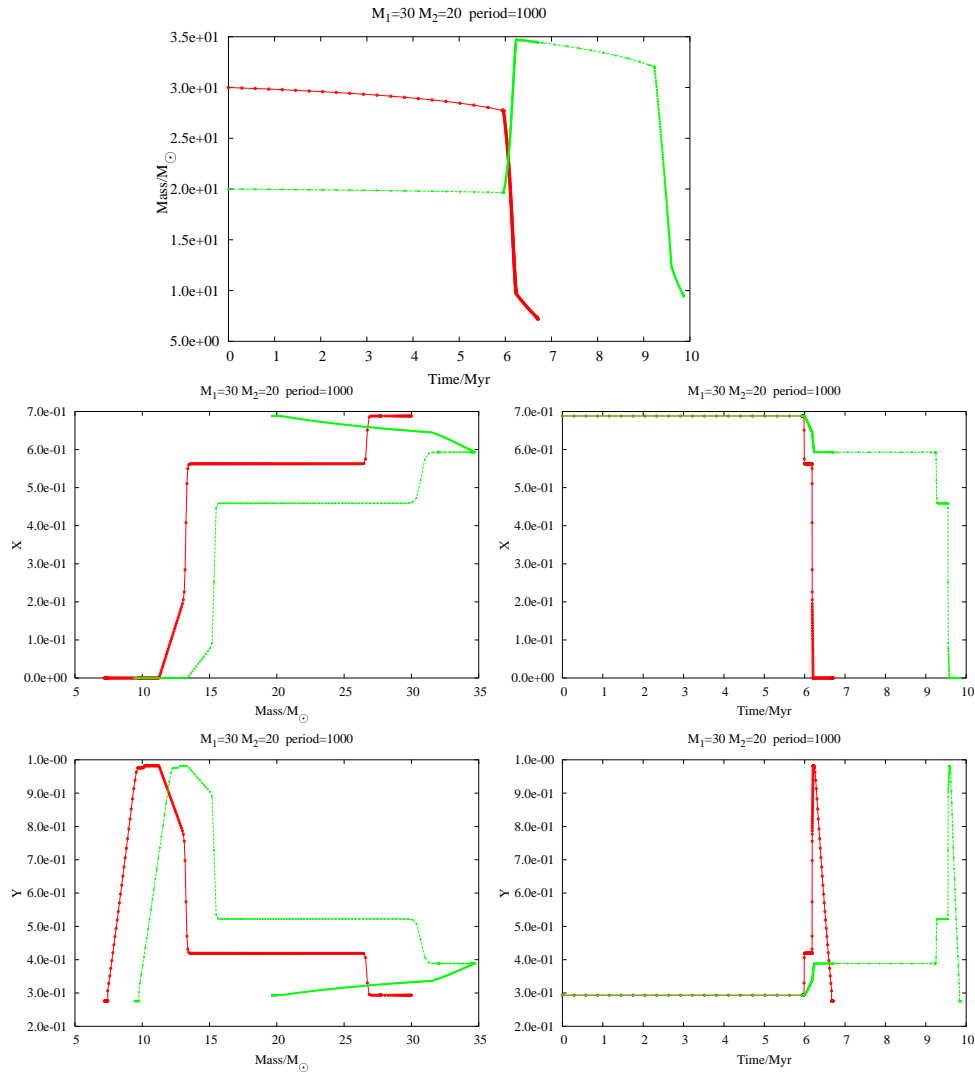
Figure 51: Stellar mass vs time, surface abundances X_{\text{H1}} , X_{\text{He4}} vs instantaneous mass and 112 vs time for a binary with initial parameters M_1 = 30 M_{\odot} , M_2 = 20 M_{\odot} and P = 1000 d (MM wind loss). Star 1 is red, star 2 is green.
