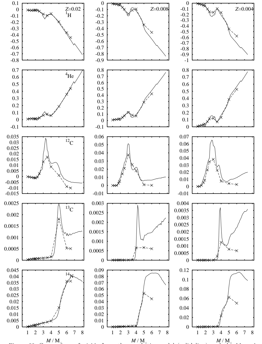
Figure 32: Comparison of yields from the synthetic model (solid line) and the Monash yields (dashed line with crosses) for Z = 0.02 , 0.008 and 0.004 , isotopes ^1\text{H} to ^{14}\text{N} .
