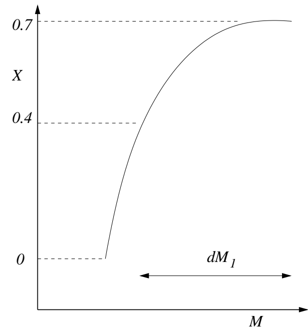
Figure 37: Schematic view of the change in surface hydrogen abundance for M \gtrsim 55 M_{\odot} .
