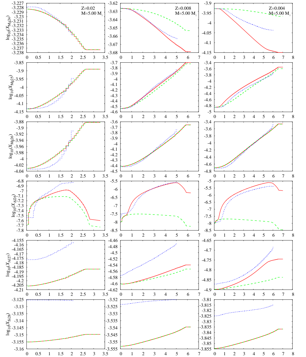
Figure 26: ^{24}\text{Mg} , ^{25}\text{Mg} , ^{26}\text{Mg} , ^{26}\text{Al} , ^{27}\text{Al} and ^{28}\text{Si} vs time for the synthetic models _{61} with MgAl chain (red), synthetic models without MgAl chain (green) and the Monash models (blue) M = 5 M_{\odot} .
