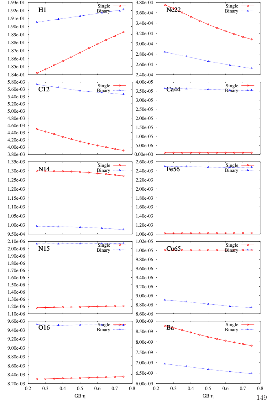
Figure 63: Yield relative to mass input y vs GB wind factor \eta .
