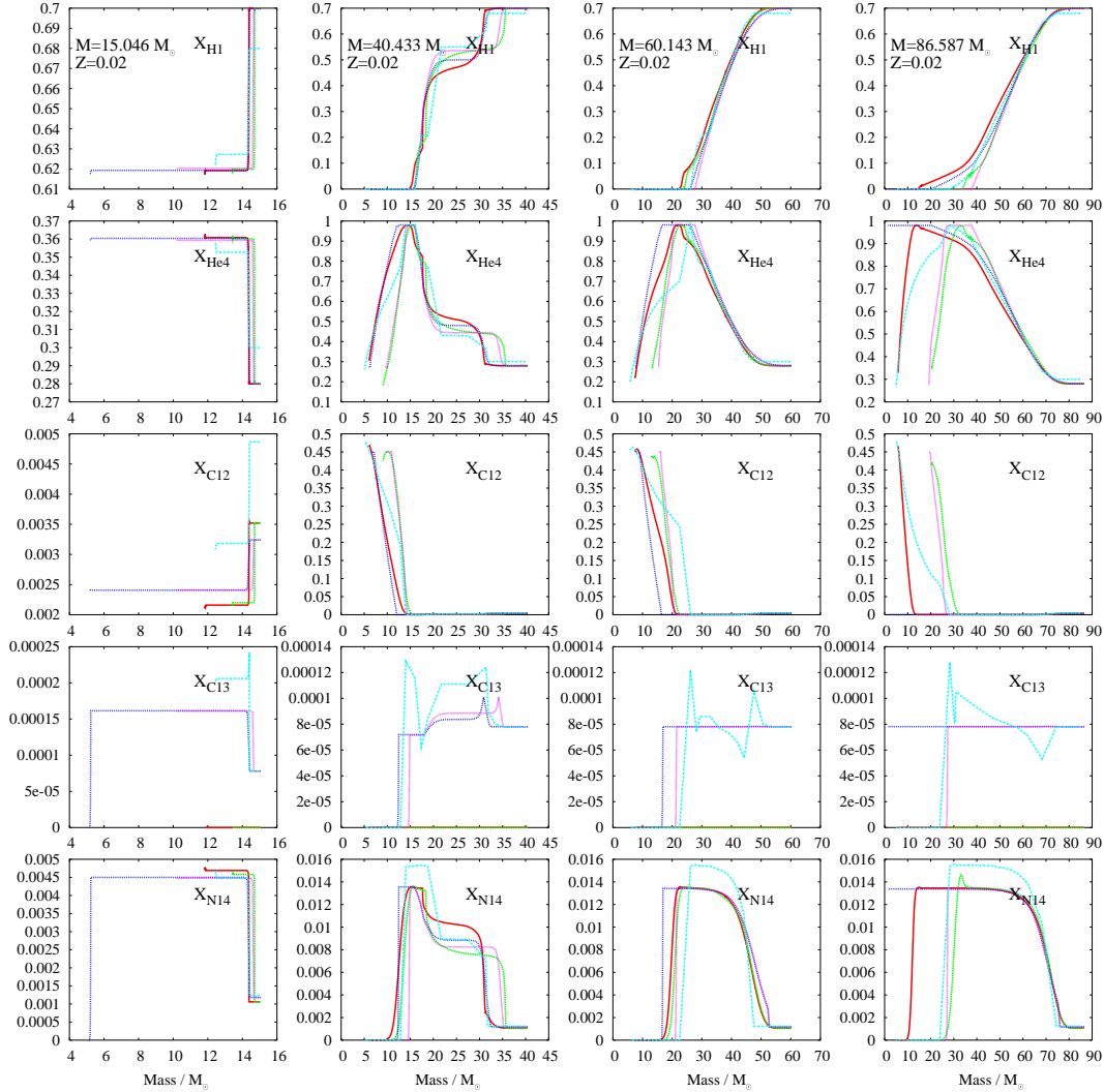
Figure 38: Comparison of surface isotopic abundances ( X_{\text{H1}} , X_{\text{He4}} , X_{\text{C12}} , X_{\text{C13}} and X_{\text{N14}} ) vs mass for Z = 0.02 and M \approx 15, 40, 60 and 86 M_{\odot} ( 85 M_{\odot} for MM94) models. The number in the top panel gives the Dray/synthetic model mass, the nearest available MM94 model is used. Red and green are the Dray models with the MM and NL mass loss rates, blue and magenta are the corresponding synthetic models, cyan are the MM94 models.
