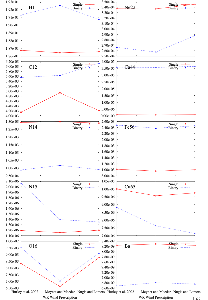
Figure 65: Yield relative to mass input y vs WR wind prescription.
