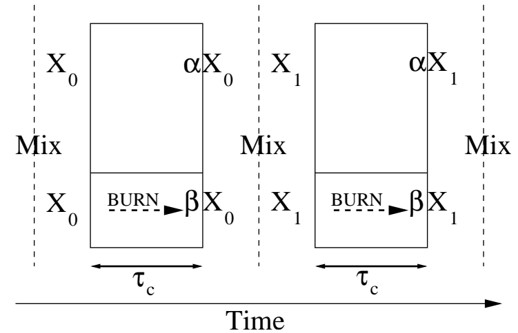
Figure 10: Synthetic convective mixing approximation: the region at the base of the envelope burns isotopes X to \beta X while radioactive decay in the envelope converts abundances X to \alpha X .
