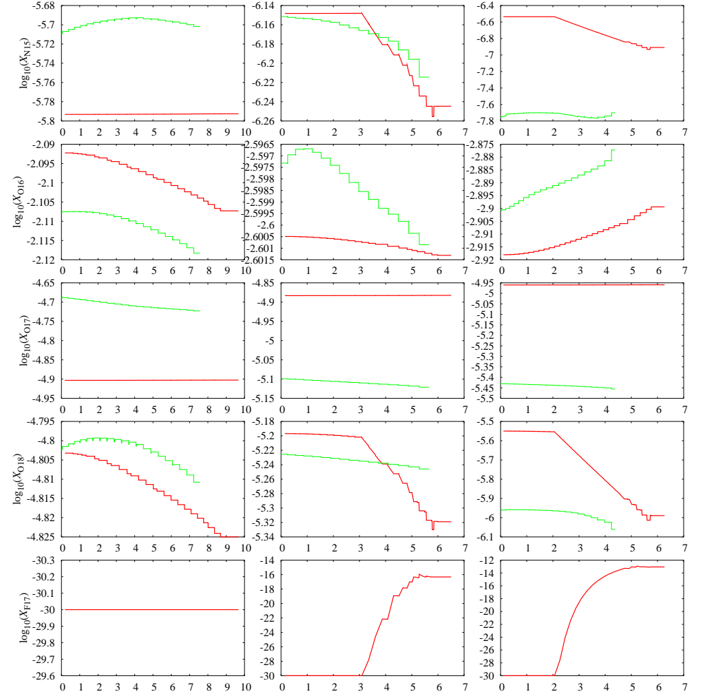
Figure 18: ^{15}\text{N} , ^{16}\text{O} , ^{17}\text{O} , ^{18}\text{O} and ^{17}\text{F} vs time (in units of 10^5 years) for the synthetic models (red) and the Monash models (green) with M = 3.5 M_{\odot} .
